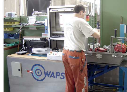
WAPS railway point drive test bench
